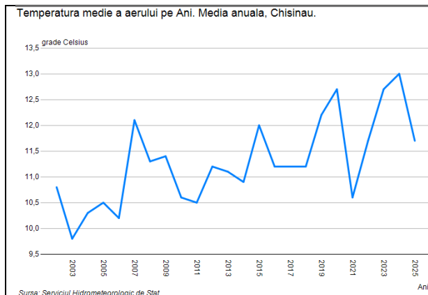
Fig. 9: Average air temperature for years 2002 - 2025
