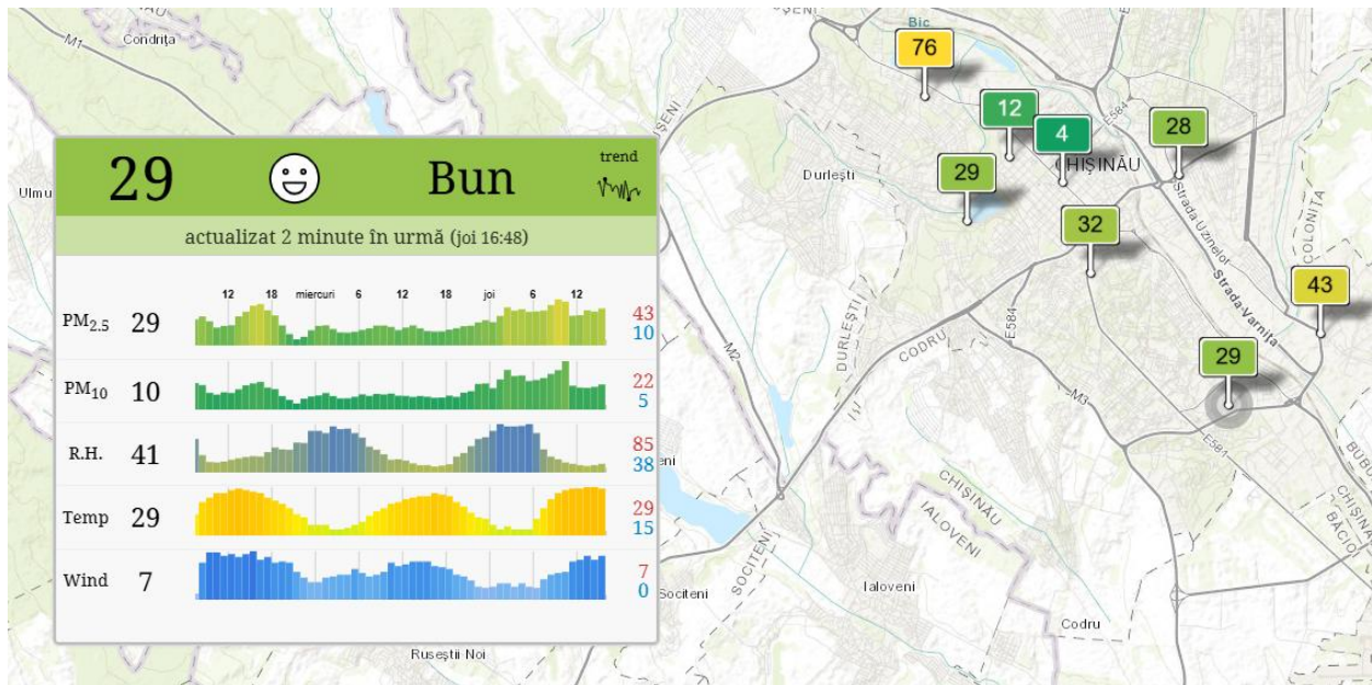
Figure 8: Real-time measurement of the concentration of pollutants in the Botanica District
