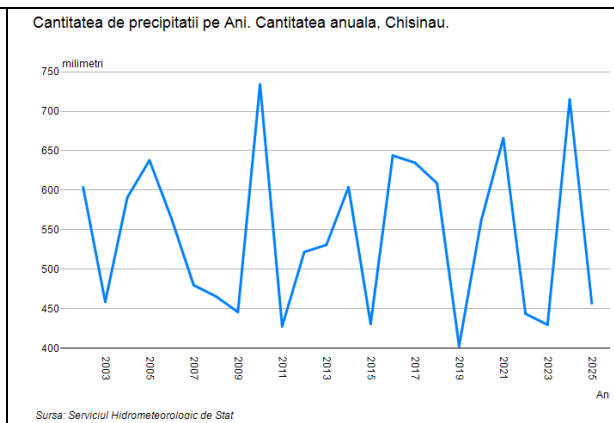
Fig. 10: Amount of precipitation for years 2002 - 2025
